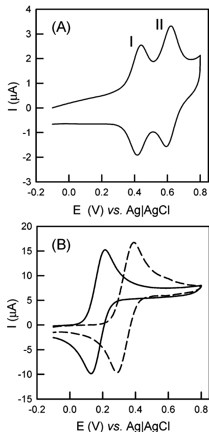
Figure 1. (A) Cyclic voltammogram recorded at a graphite electrode covered with 1.0\ \mu\text{L} of nitrobenzene ( NB ) containing 0.11\text{ mM} DFcB . The supporting electrolyte was 0.1\text{ M} tetraethylammonium perchlorate (TEAP) in the NB phase; 0.1\text{ M NaCl} + 0.1\text{ M NaClO}_4 in the aqueous phase. The scan rate was 10\text{ mV/s} . (B) Cyclic voltammograms recorded at a bare graphite electrode in 1.0\text{ mM} [\text{Fe}(\text{CN})_6]^{4-} . Supporting electrolytes: 0.1\text{ M NaCl} + 0.1\text{ M NaClO}_4 (solid line), 0.1\text{ M HCl} + 0.1\text{ M NaClO}_4 (dashed line). The scan rate was 5\text{ mV/s} .
