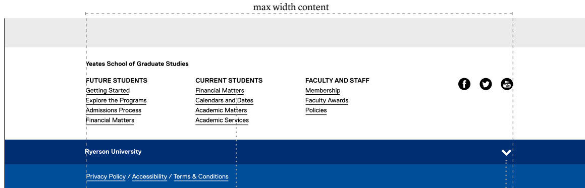
Global Footer: Collapsed (desktop)
